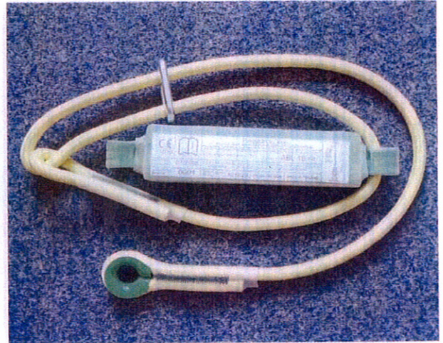
Fig. of the Energy absorber with lanyard, type ABL-16 FR
